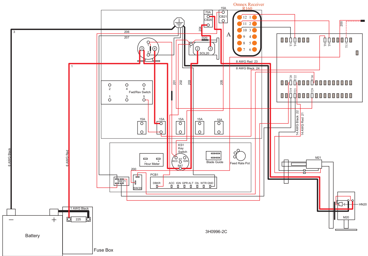
FIG. 5-12
