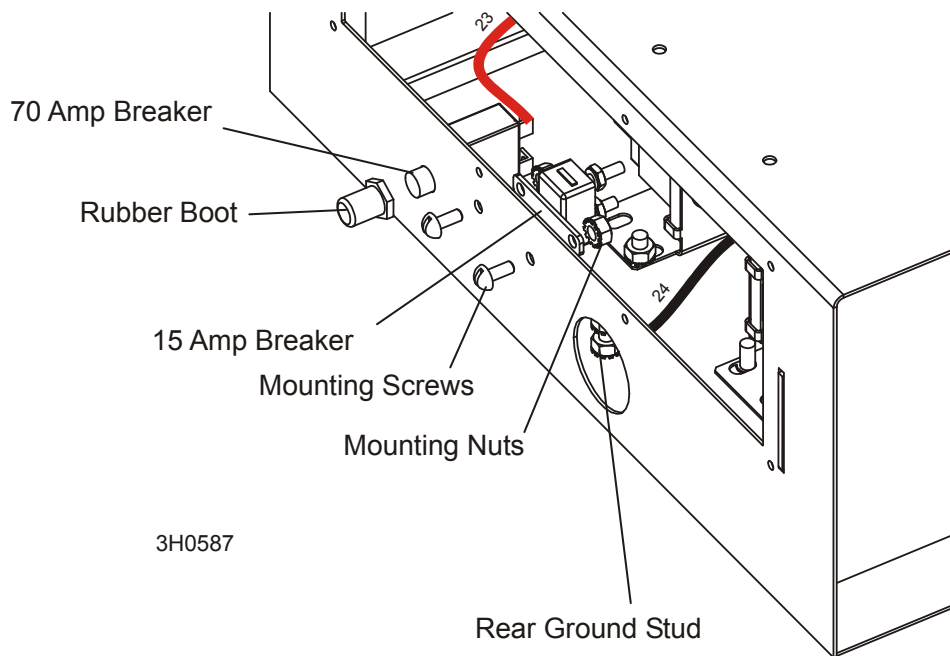
FIG. 2-8 LT60HD/70HD (BEFORE 9/04)
