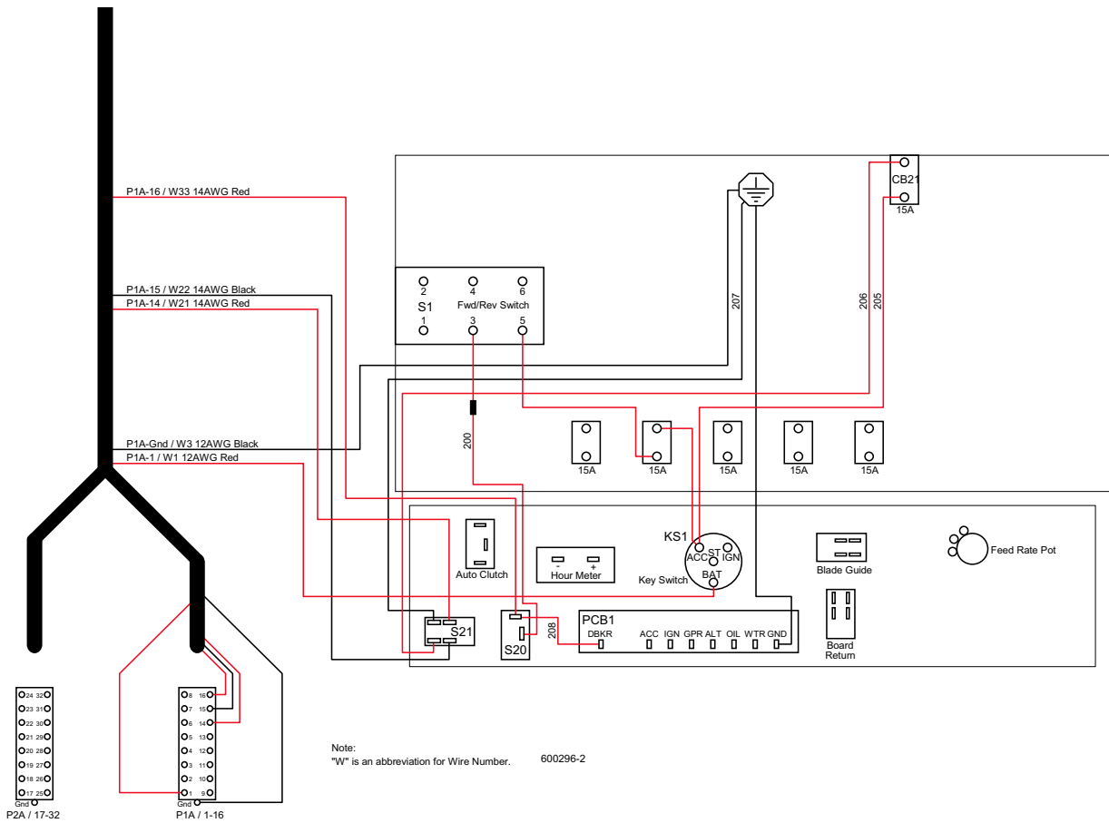
FIG. 5-7 (PAGE 2 OF 2)
