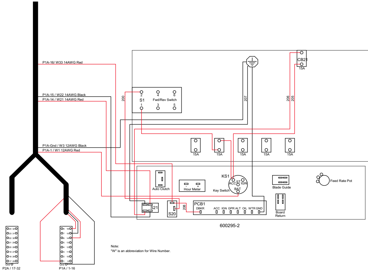
FIG. 5-11 (PAGE 2 OF 2)
