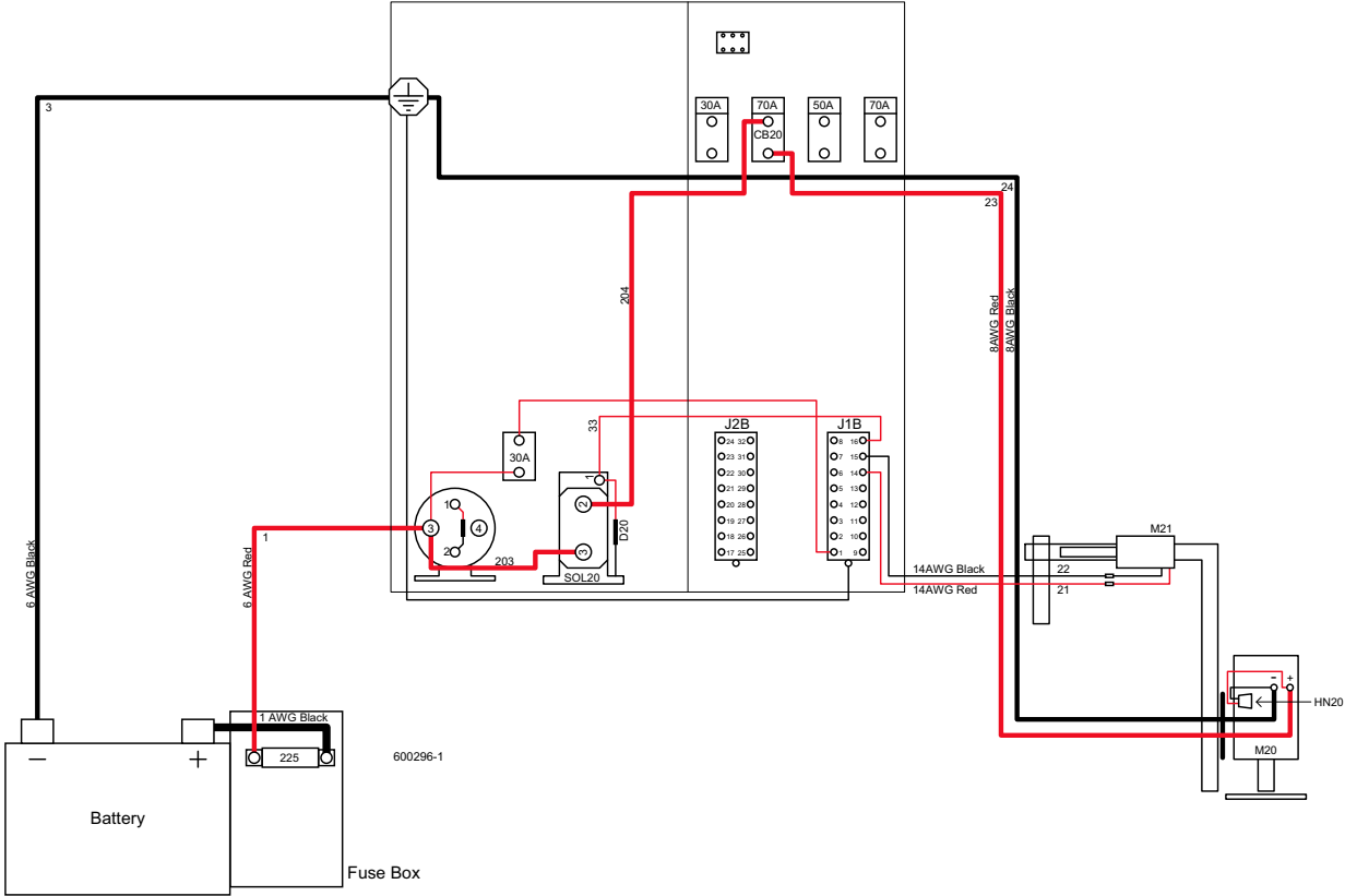
FIG. 5-8 (PAGE 1 OF 2)
