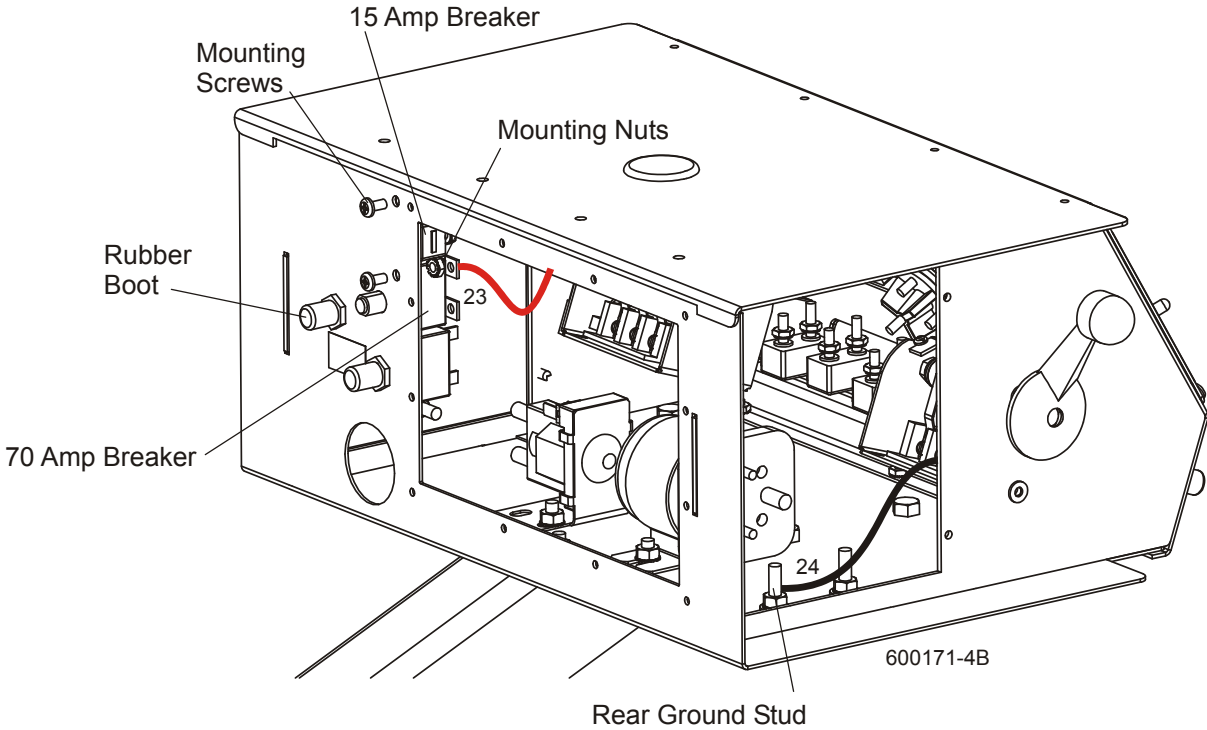
FIG. 2-8 LT60HD/70HD(AFTER 9/04)
