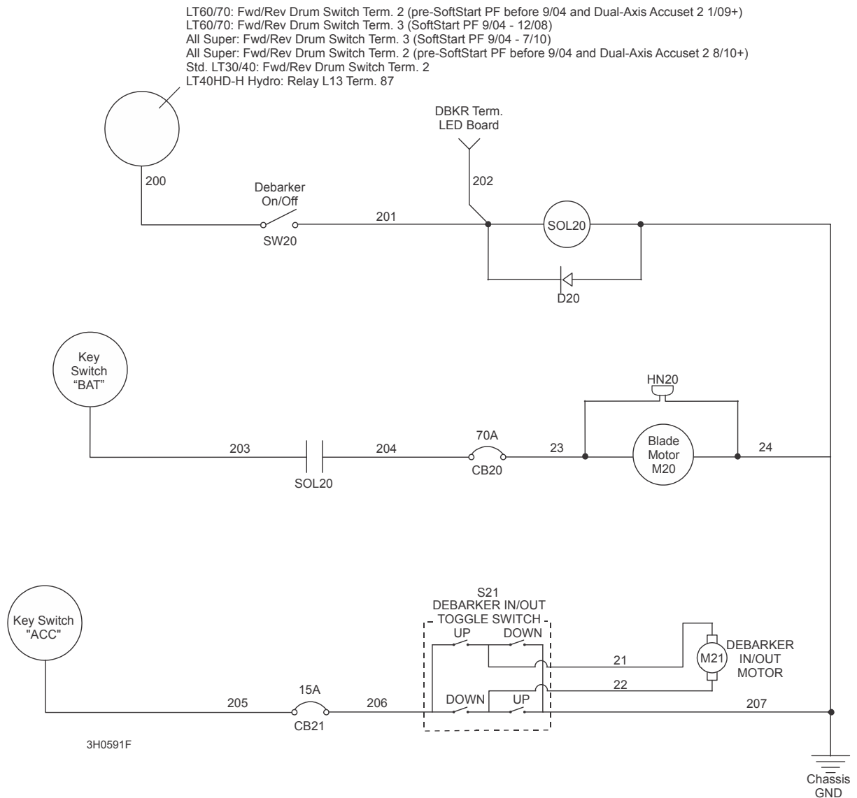
FIG. 5-1 NON-REMOTE SAWMILL
