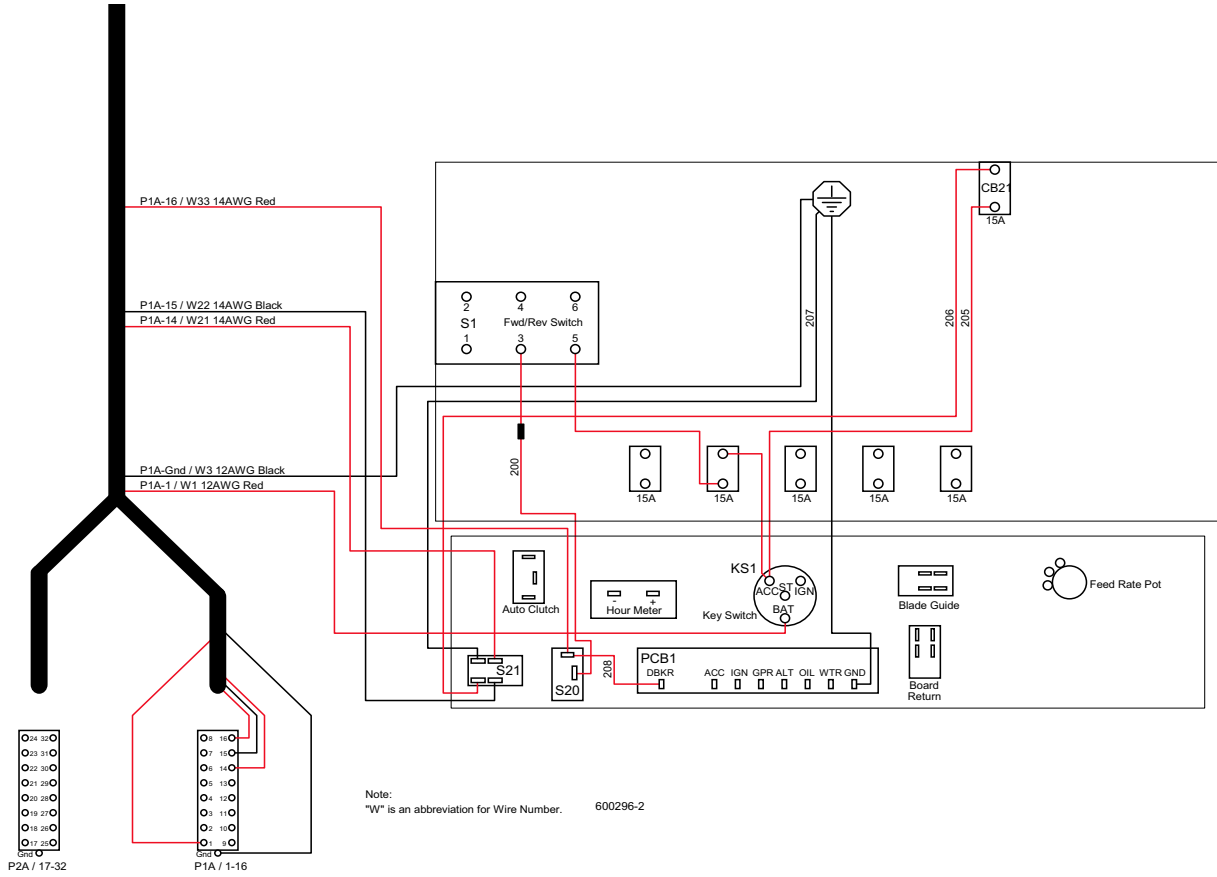
FIG. 5-9 (PAGE 2 OF 2)
