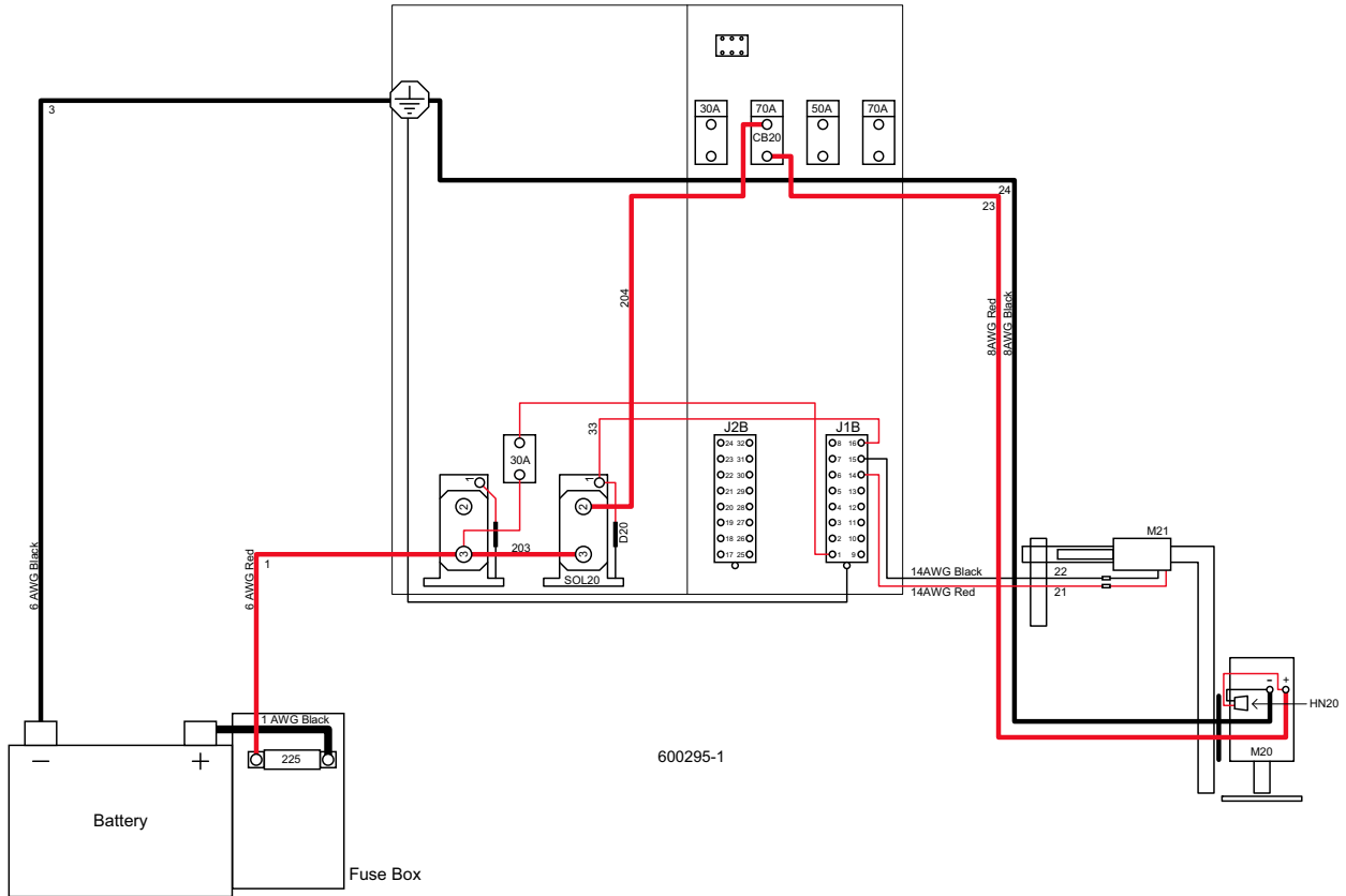
FIG. 5-10 (PAGE 1 OF 2)
