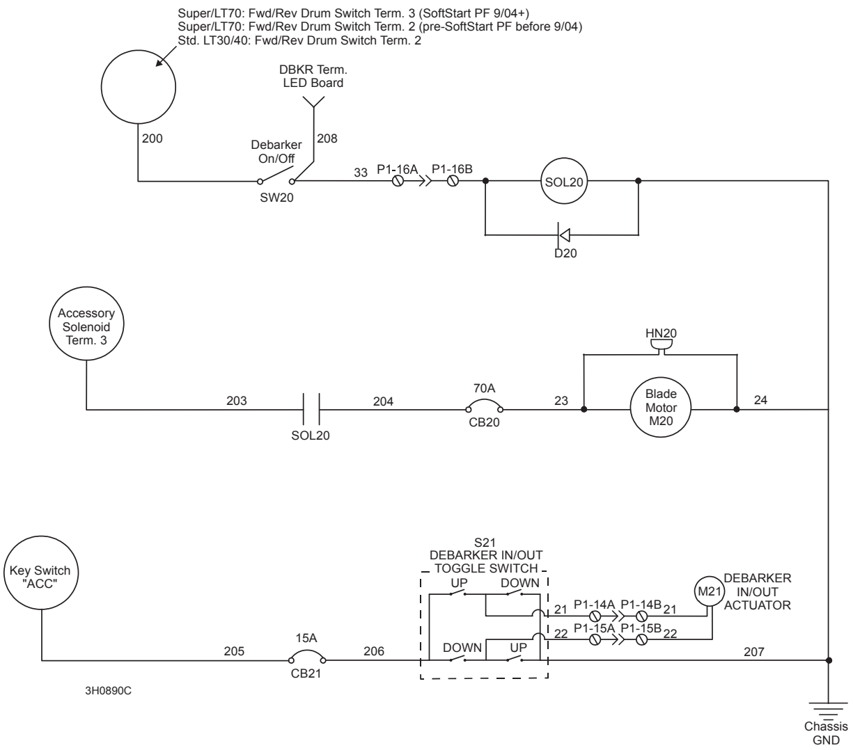
FIG. 5-2 REMOTE SAWMILL
