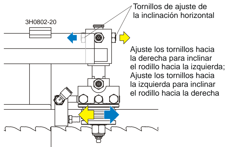
FIGURA 7-11 PRIOR TO REV. K1.01
