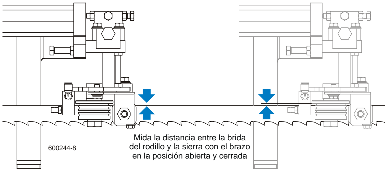
FIGURA 7-4 REV. K1.01 - K3.02 (OPTIONAL HIGH-PERFORMANCE ROLLER/BLOCKS SHOWN)
