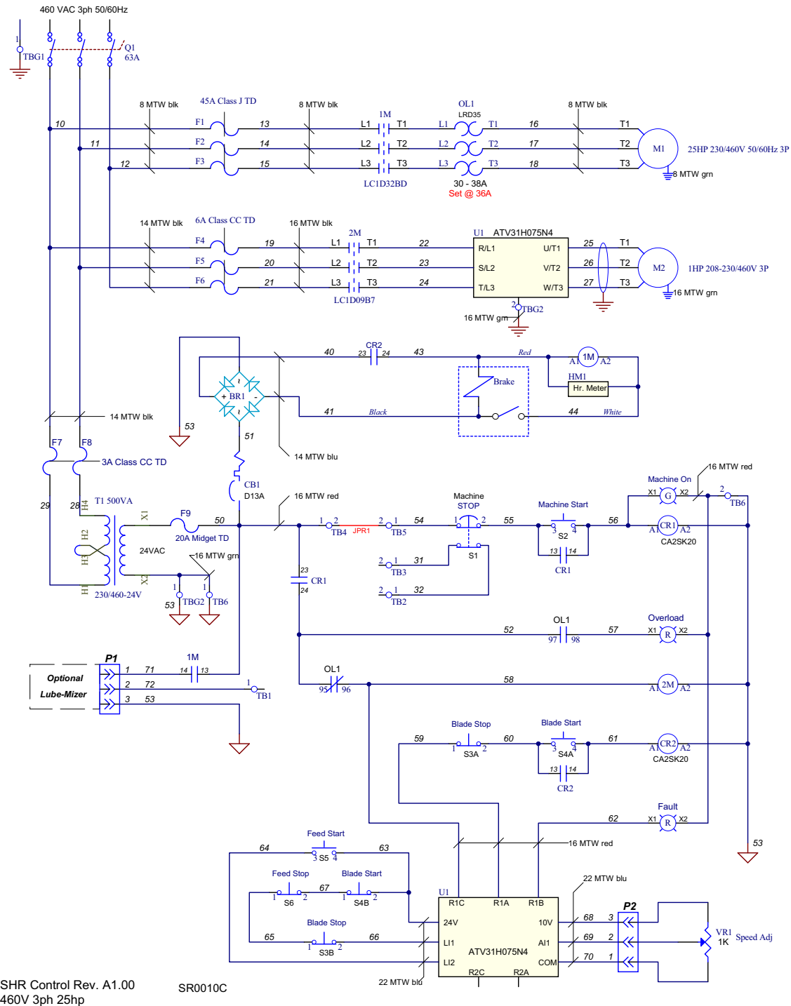
FIG. 1-13 SYMBOL DIAGRAM ()
