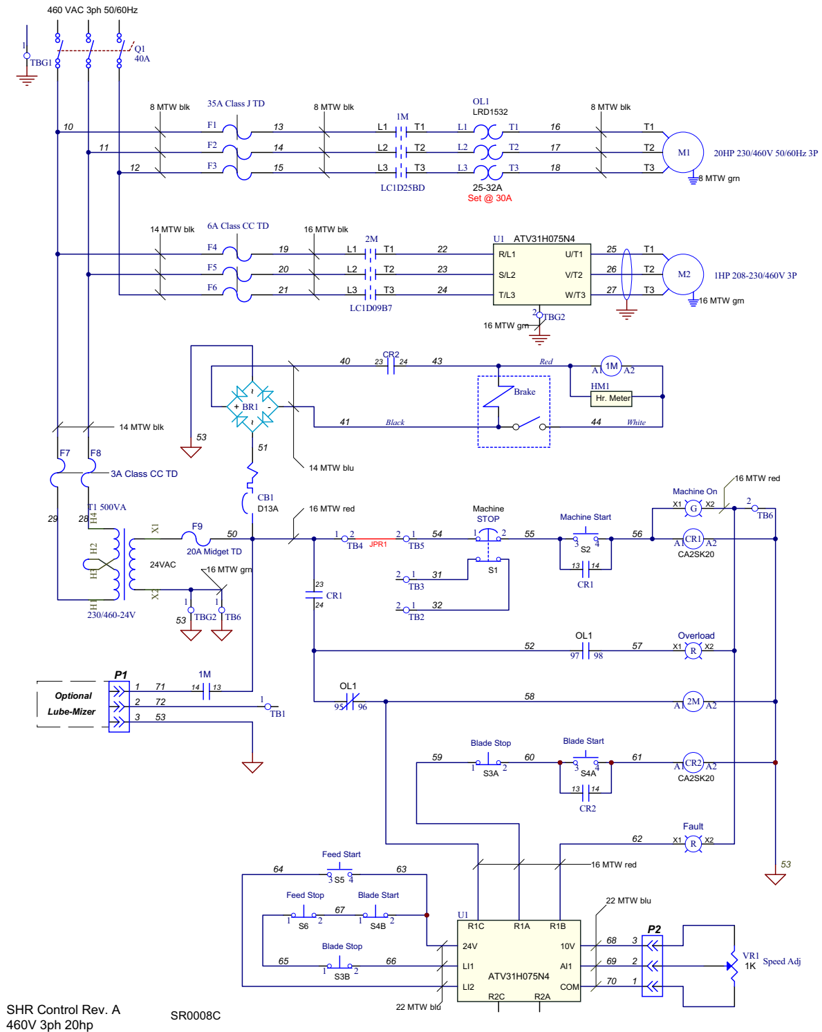
FIG. 1-10 SYMBOL DIAGRAM ( )
