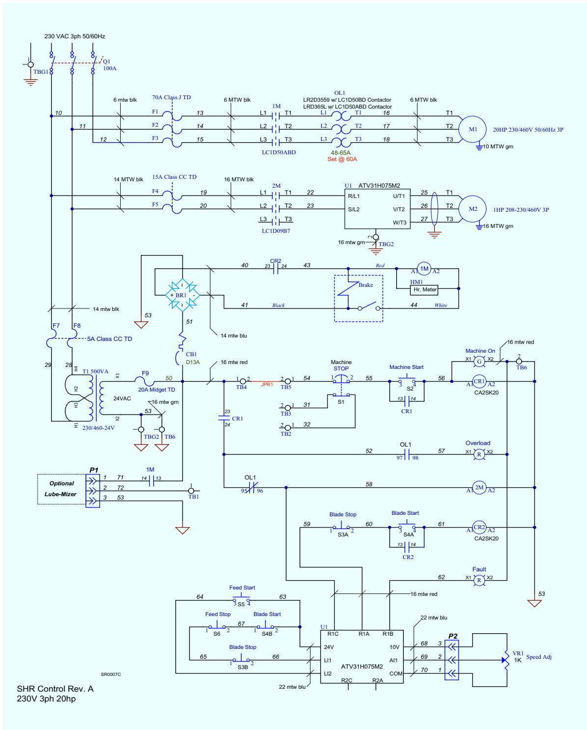
FIG. 1-9 SYMBOL DIAGRAM ( )
