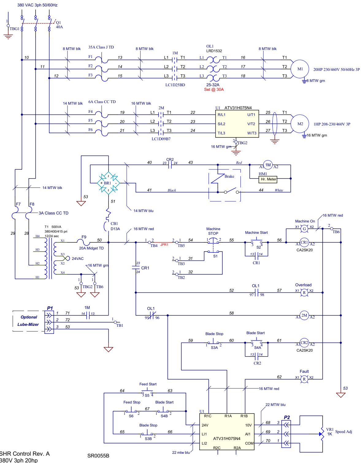
FIG. 1-11 SYMBOL DIAGRAM ()
