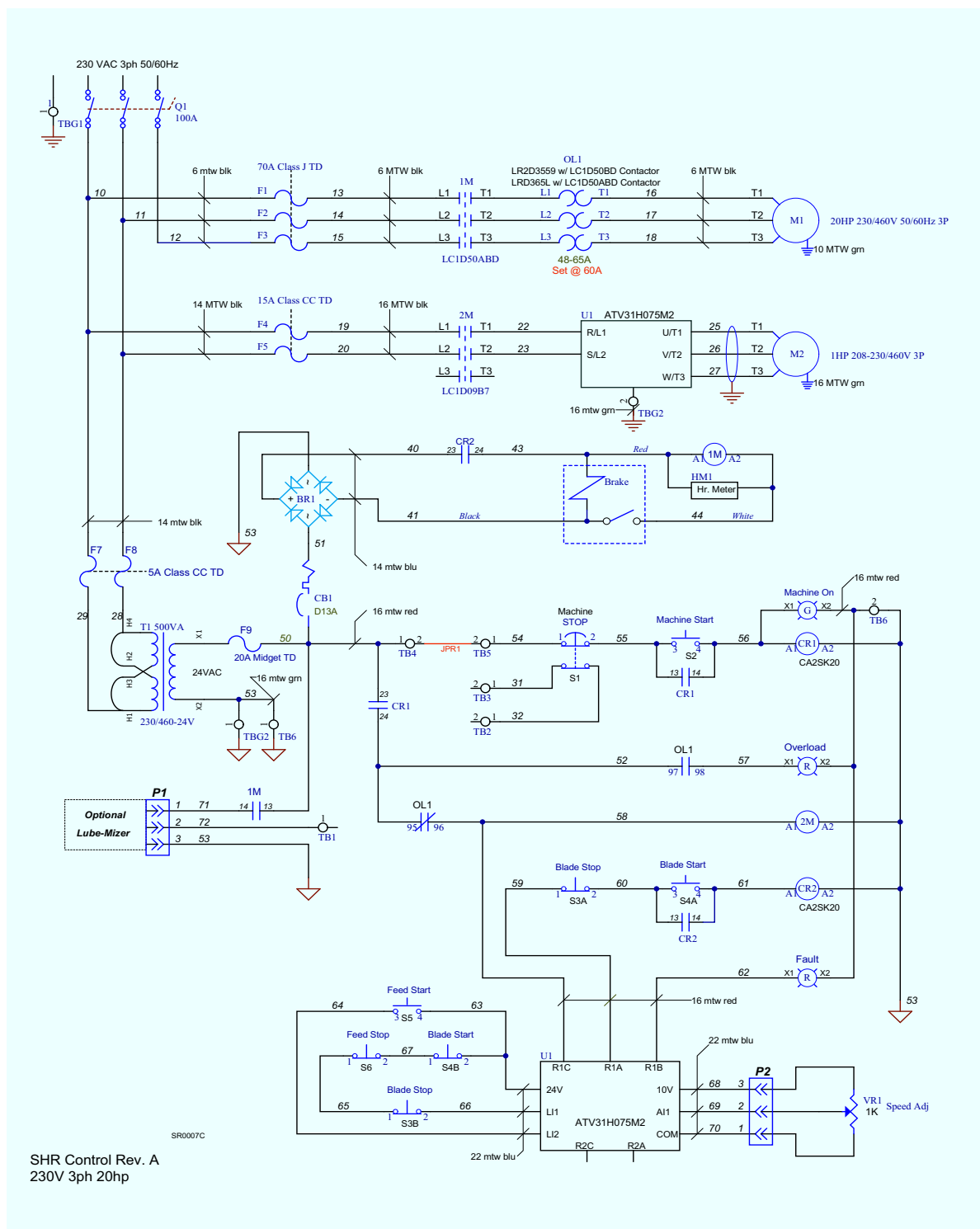
FIG. 1-9 SYMBOL DIAGRAM ()
