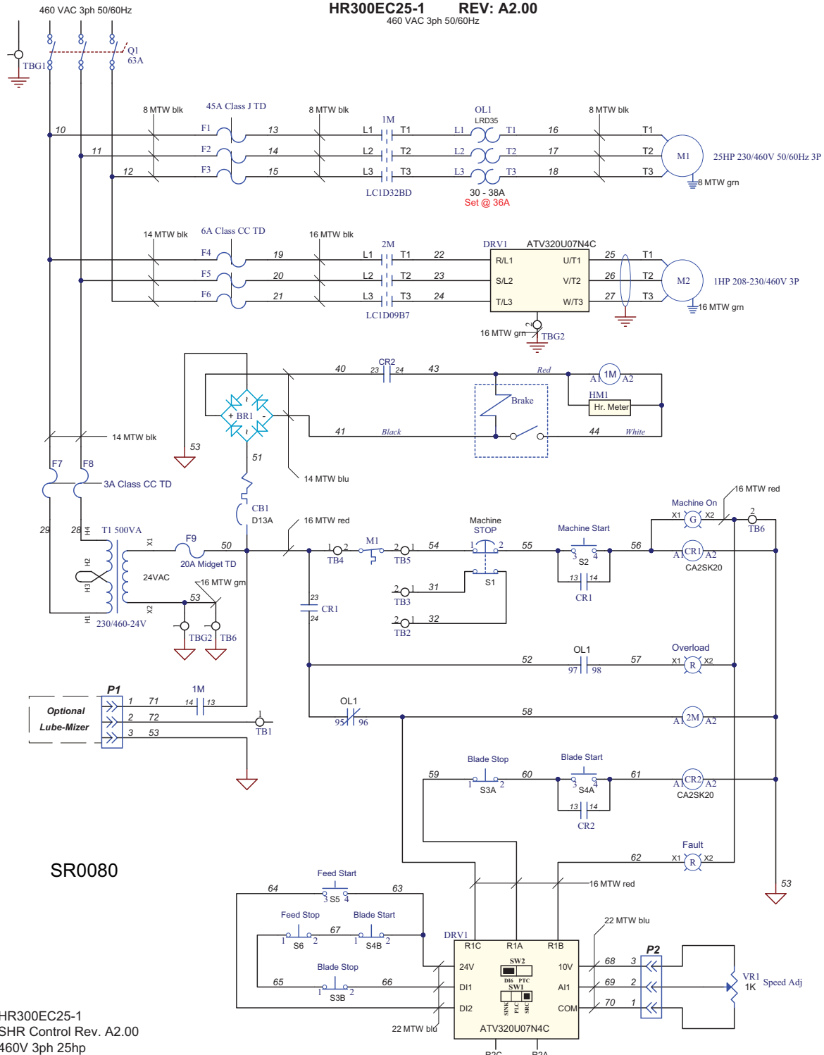
FIG. 1-6 SYMBOL DIAGRAM (HR300EC25-1)
