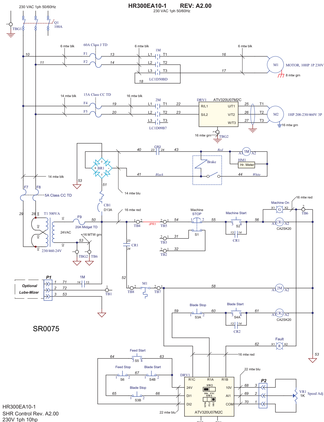
FIG. 1-1 SYMBOL DIAGRAM (HR300EA10-1)
