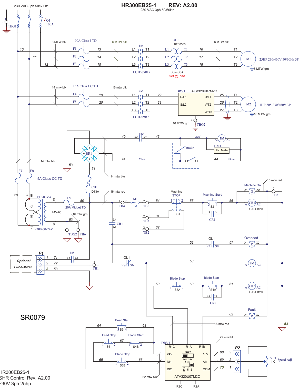
FIG. 1-5 SYMBOL DIAGRAM (HR300EB25-1)
