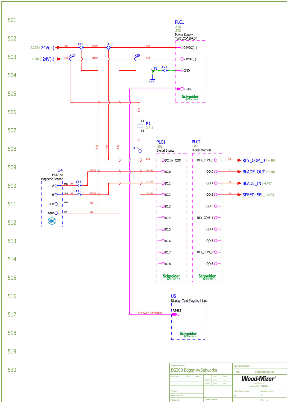
FIG. 1-5 SYMBOL DIAGRAM (EG300EC25U PAGE 5 OF 5)
