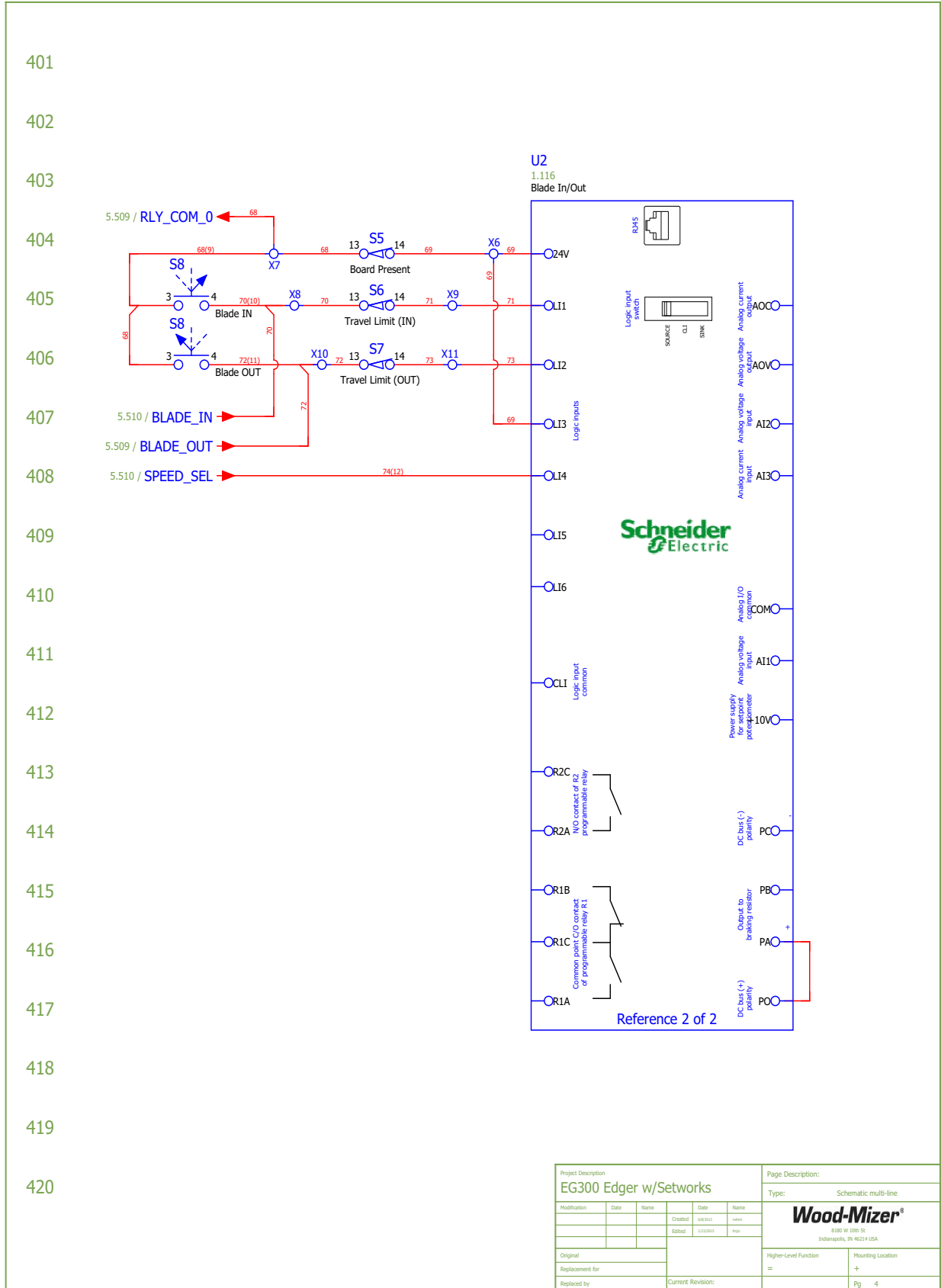
FIG. 1-4 SYMBOL DIAGRAM (EG300EC25U PAGE 4 OF 5)
