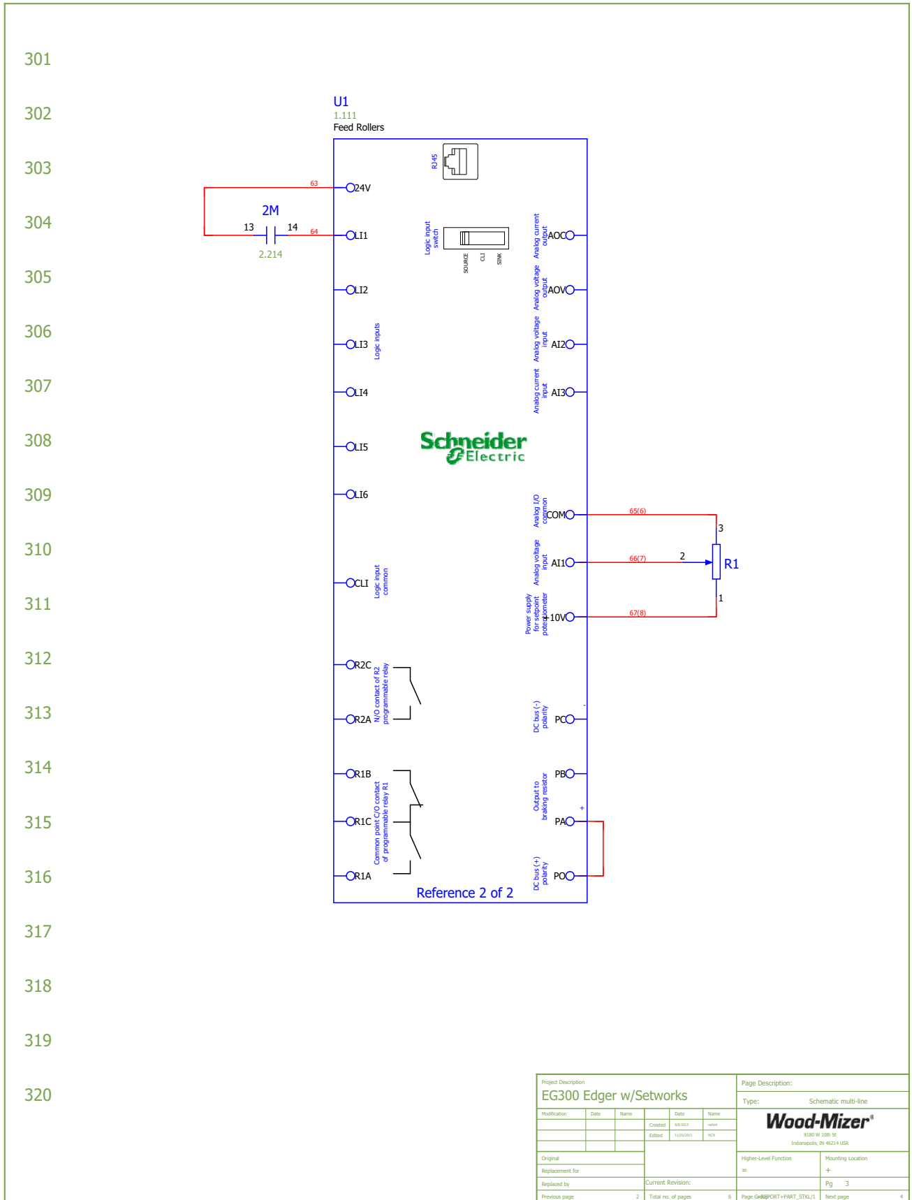
FIG. 1-3 SYMBOL DIAGRAM (EG300EC25U PAGE 3 OF 5)
