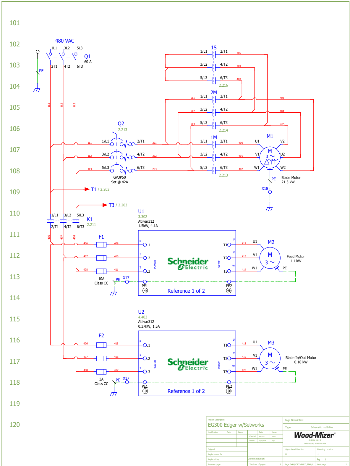
FIG. 1-1 SYMBOL DIAGRAM (EG300EC25U PAGE 1 OF 5)
