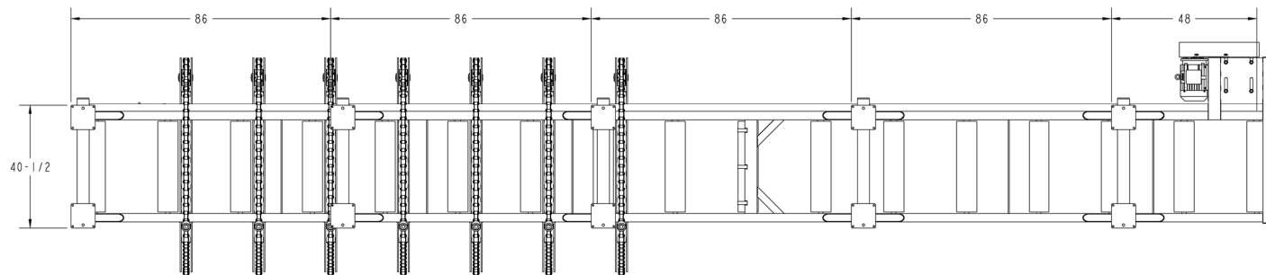
View without covers plates Chain Routing
