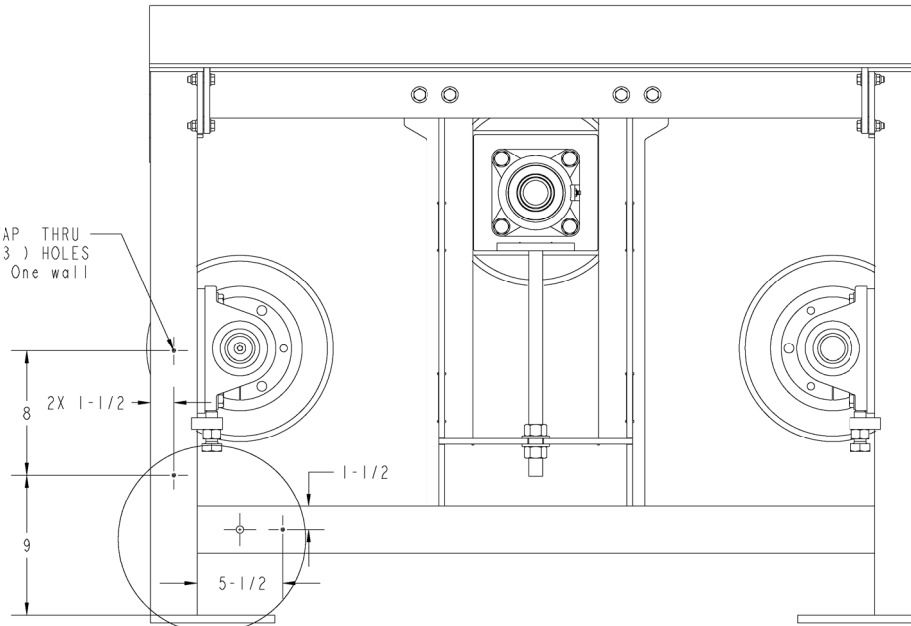
View without Assy Encoder System
