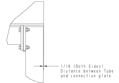
DETAIL A SCALE 0.188
