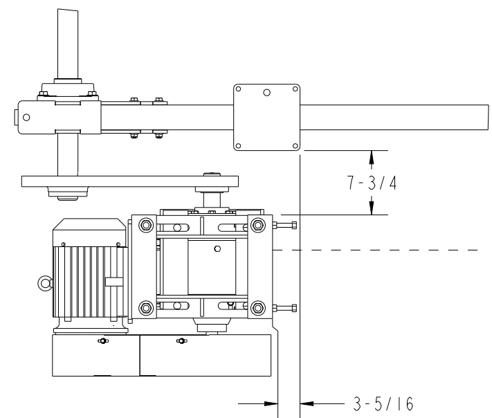
DETAIL A SCALE 0.062
