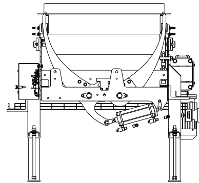
SECTION C-C SCALE 0.063
