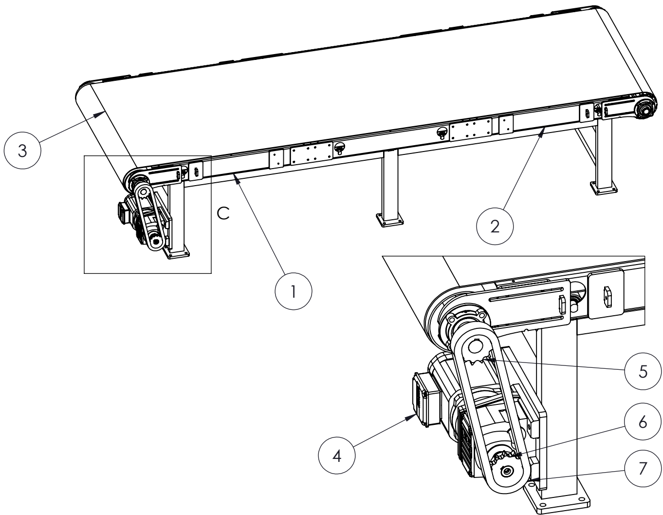
DETAIL C
