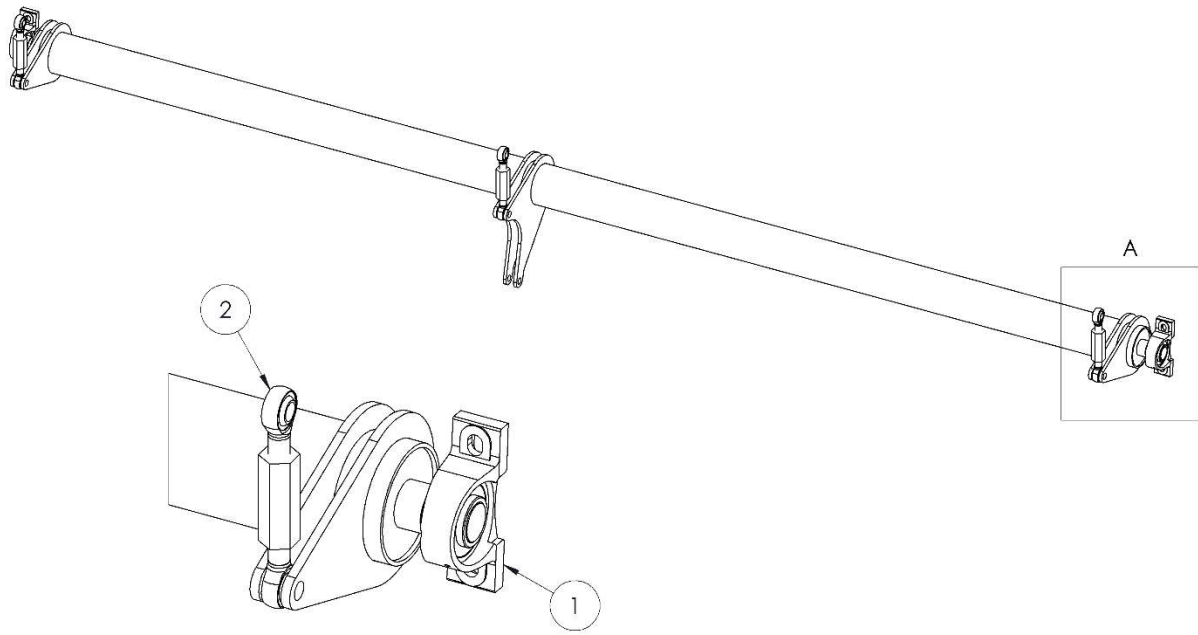
DETAIL A
