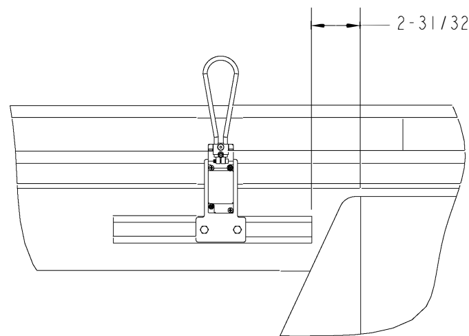
DETAIL M SCALE 0.125
