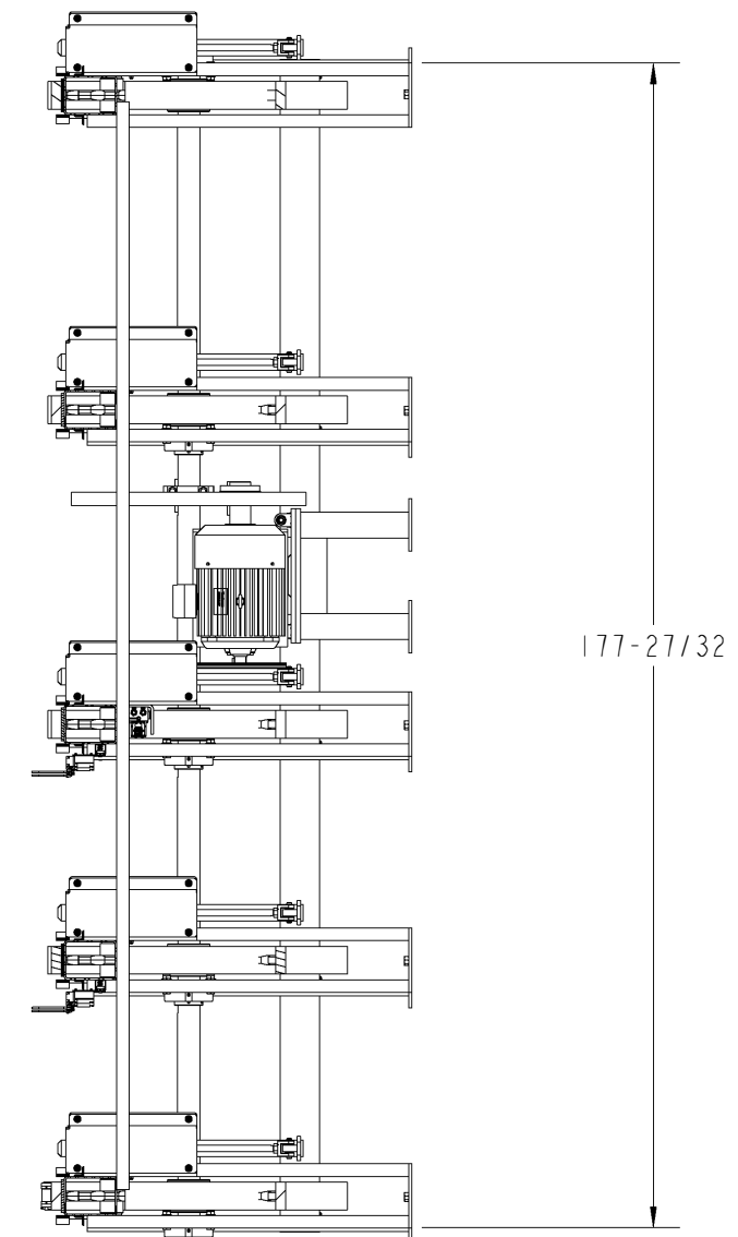
SECTION B-B
