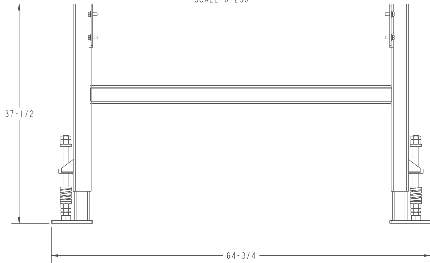
DETAIL A SCALE 0.250
