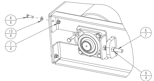
DETAIL A SCALE 0.125
