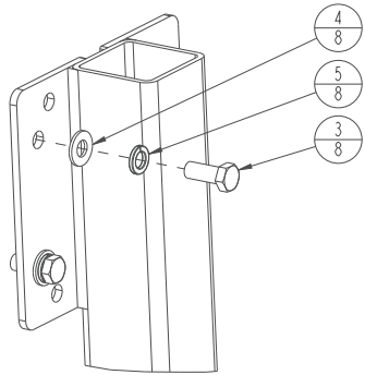
DETAIL A SCALE 0.250
