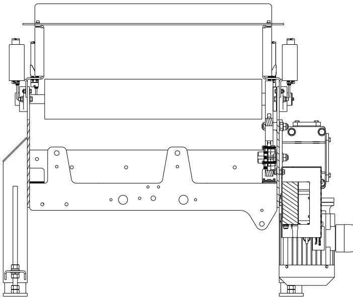
SECTION C-C SCALE 0.063
