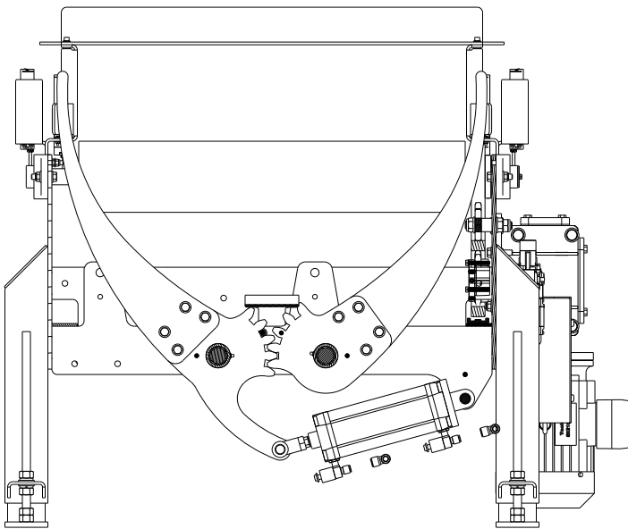
SECTION B-B SCALE 0.063
