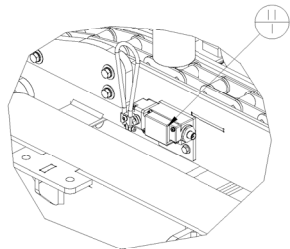
DETAIL C SCALE 0.250
