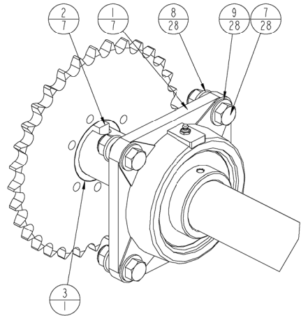
DETAIL A SCALE 0.250
